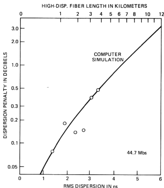
Fig. 9—Effect of RMS dispersion.
